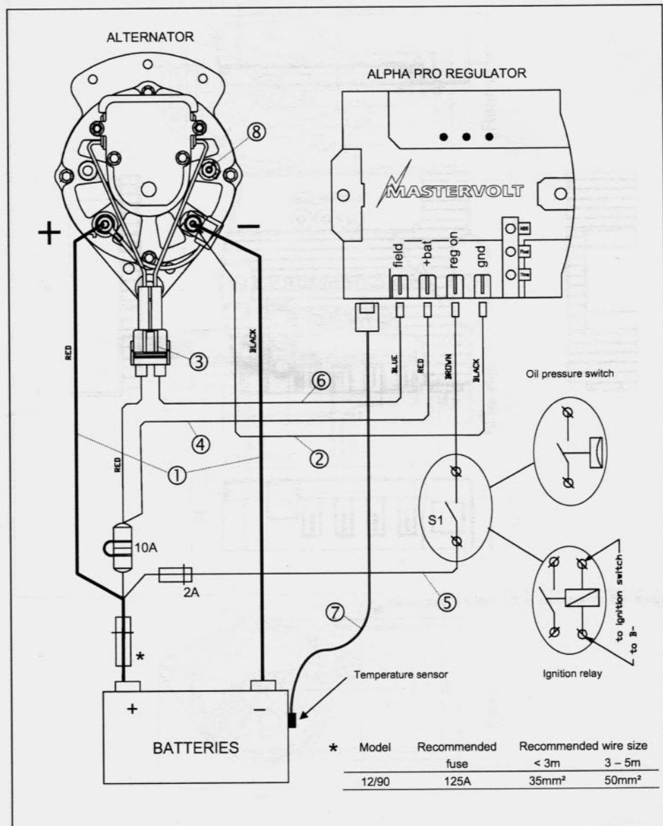
Figure A-6: Installation drawing Alpha alternator model 12/90
