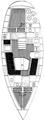
• Layout of the Oceanquest AC
